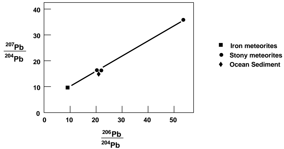
The lead isochron for ocean sediment and meteorites. The slope indicating an age of 4.54 \pm 0.07 Byr (after fig 1, C. Patterson, Geochimica et Cosmochimica Acta , Vol. 10, p:232 1956)
