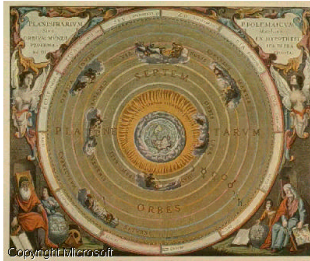
Geocentric Cosmos
