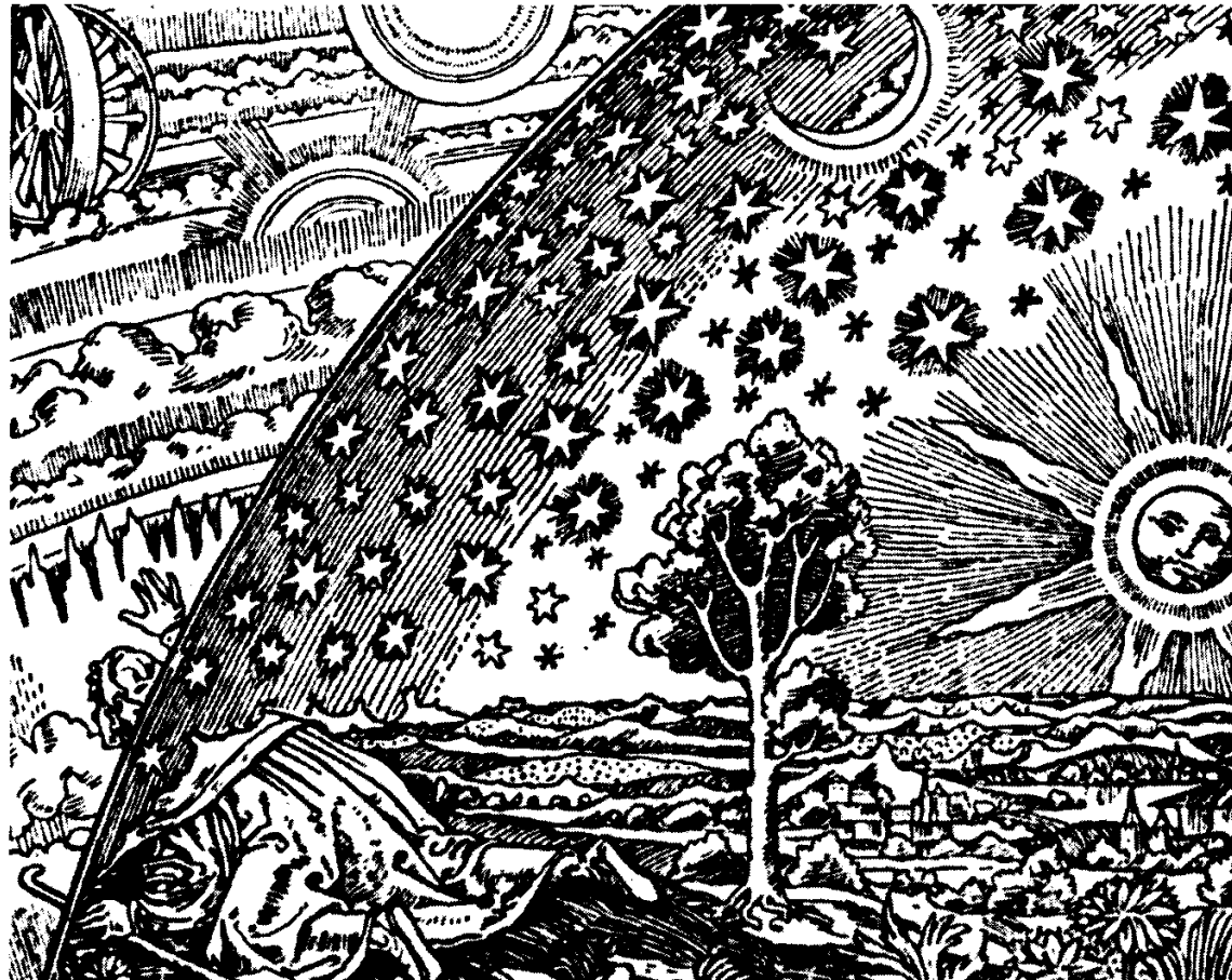
Ptolemy's Spheres
