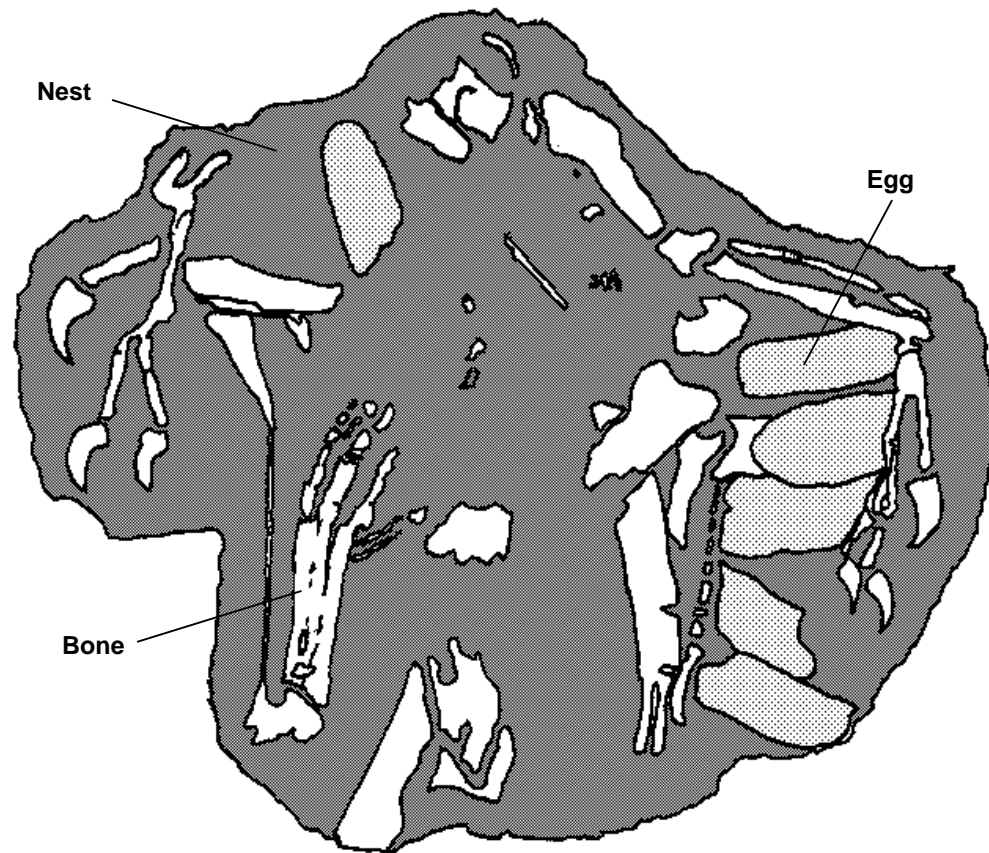
Diagrammatic representation of bones and eggs in position (after photograph, fig. 1a, Nature , Vol. 378, p:775 1995)
